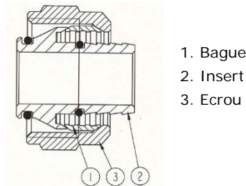
Figure 1 - Raccord à compression ROTH
